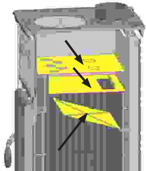
SMOKE BAFFLE
